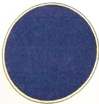
new moon
