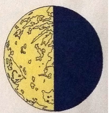
last quarter
