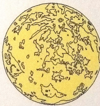
full moon
