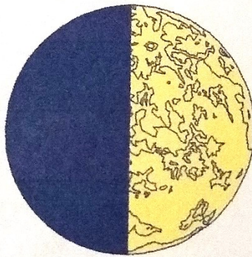
first quarter
